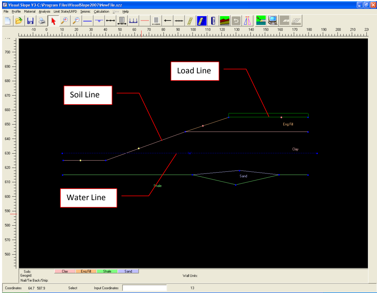
Figure 4 Typical Visual Slope Profile
