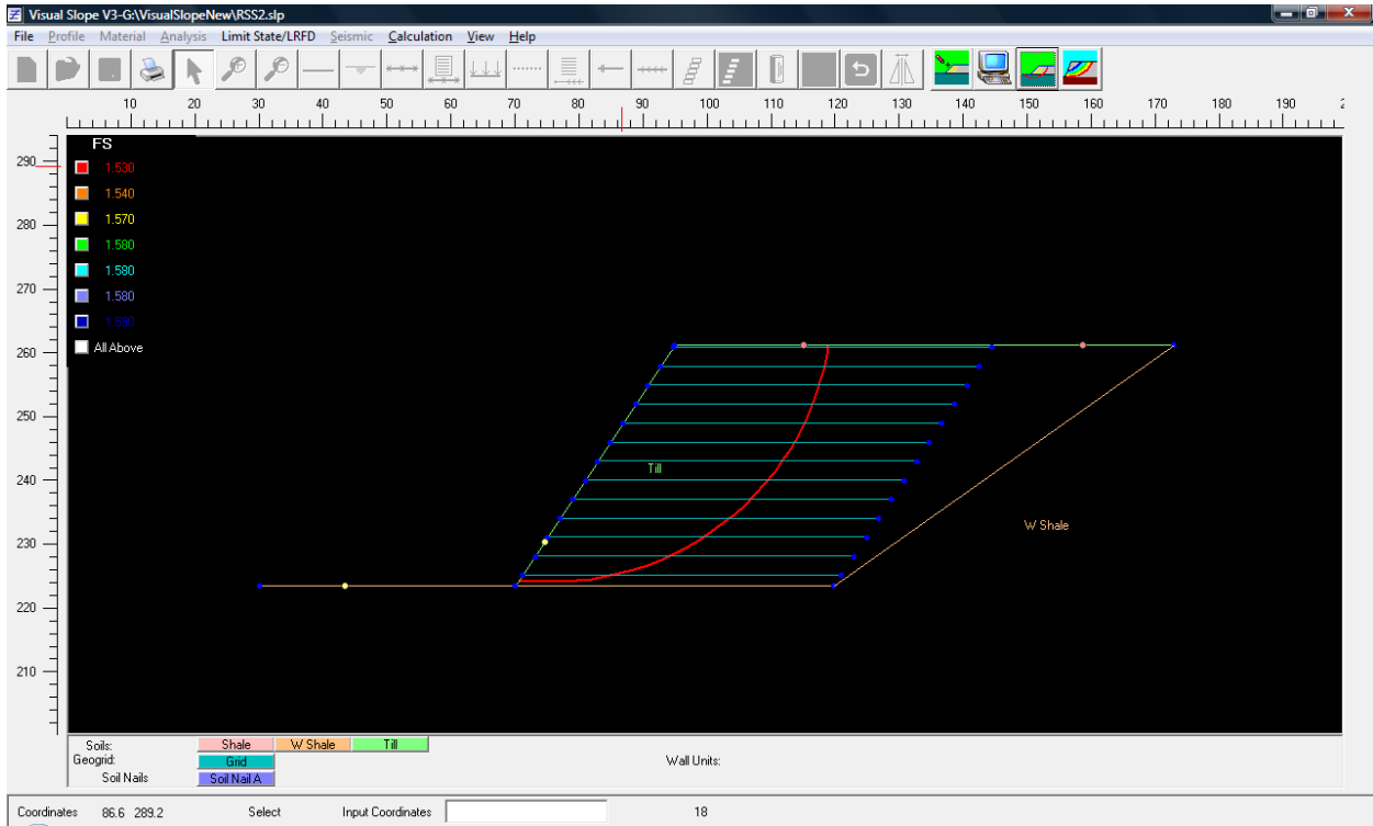
Figure 29 Circular Failure
