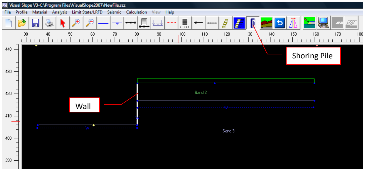
Figure 41 Retaining Wall
