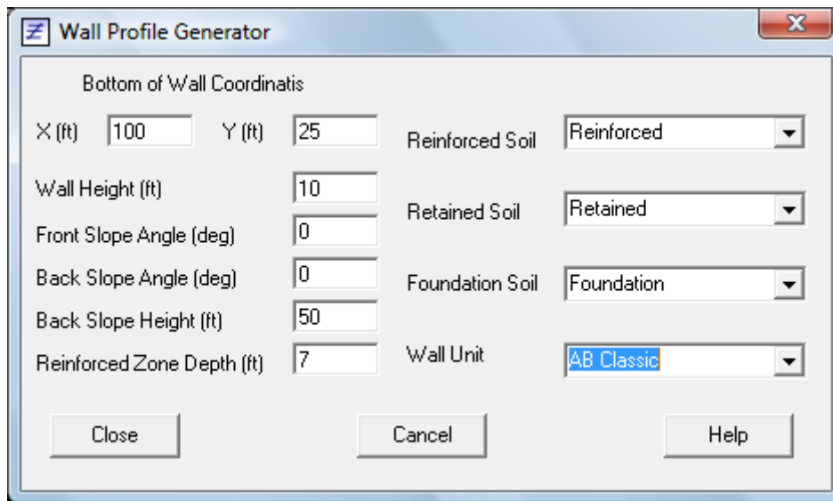
Figure 32 Wall Profile Generator
